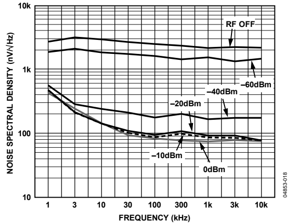
Figure 19. Noise Spectral Density of Output; CLPF = Open
